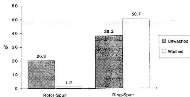
Exhibit 7: Average percentage change in lint grade with combing, rotor vs. ring spinning, before and after washing
